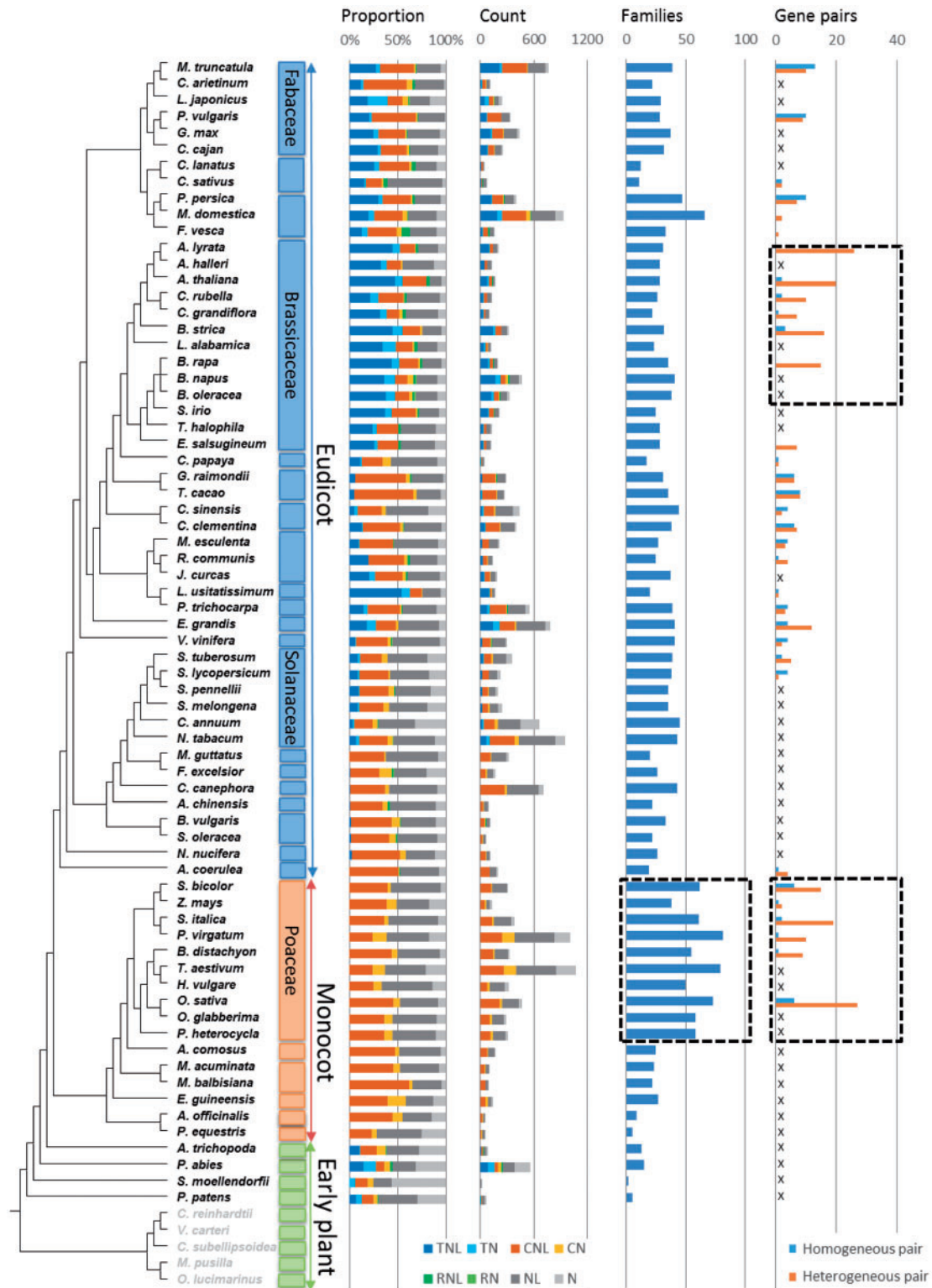
FIG. 1. Variation in copy number and composition of NBS genes in 75 plant genomes. The four bar charts, from left to right, represent for each genome the proportion of different types of NBS genes, the total number or count of NBS genes, the number of NBS families and convergent/divergent NBS pairs. The black boxes signify that total number of NBS families in the Poaceae and the number of heterogeneous pairs of NBS genes in the Poaceae and Brassicaceae is much higher than those in other genomes. In the chart for gene pairs, missing data are denoted with an “X” mark and is due to short genomic assemblies or the lack of a usable or complete gene annotation file.
